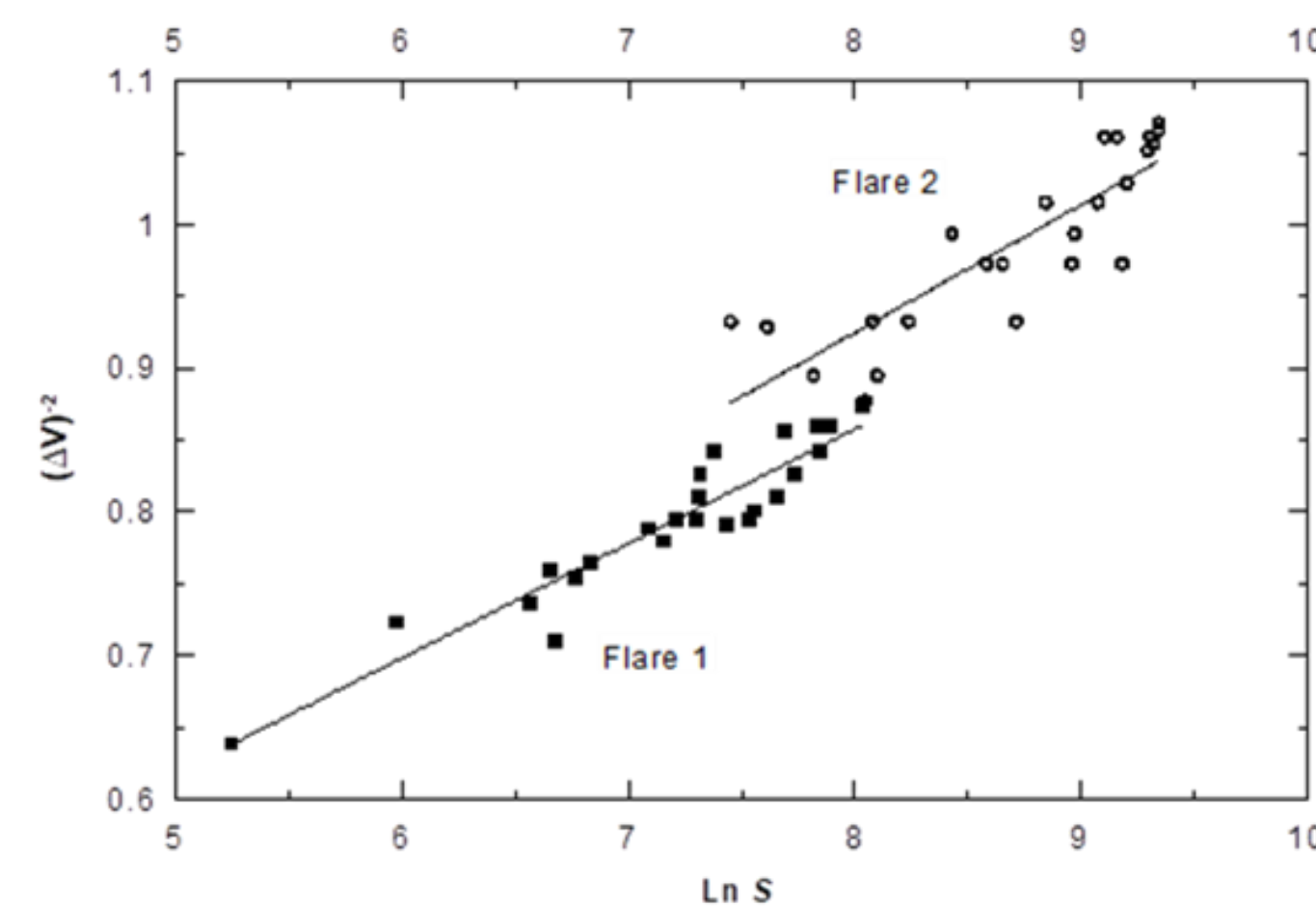
Fig. The dependencies between (\Delta v)^{-2} and \ln(S) .
